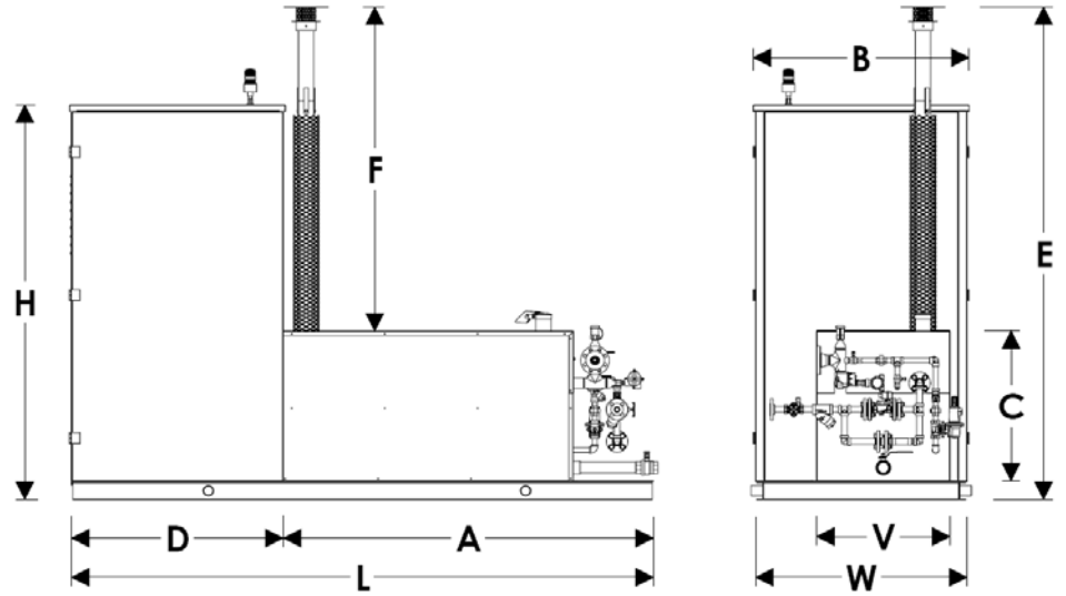
Dimensions for all 08-Series Vaporizers with Full-Size Step-in Control Room
