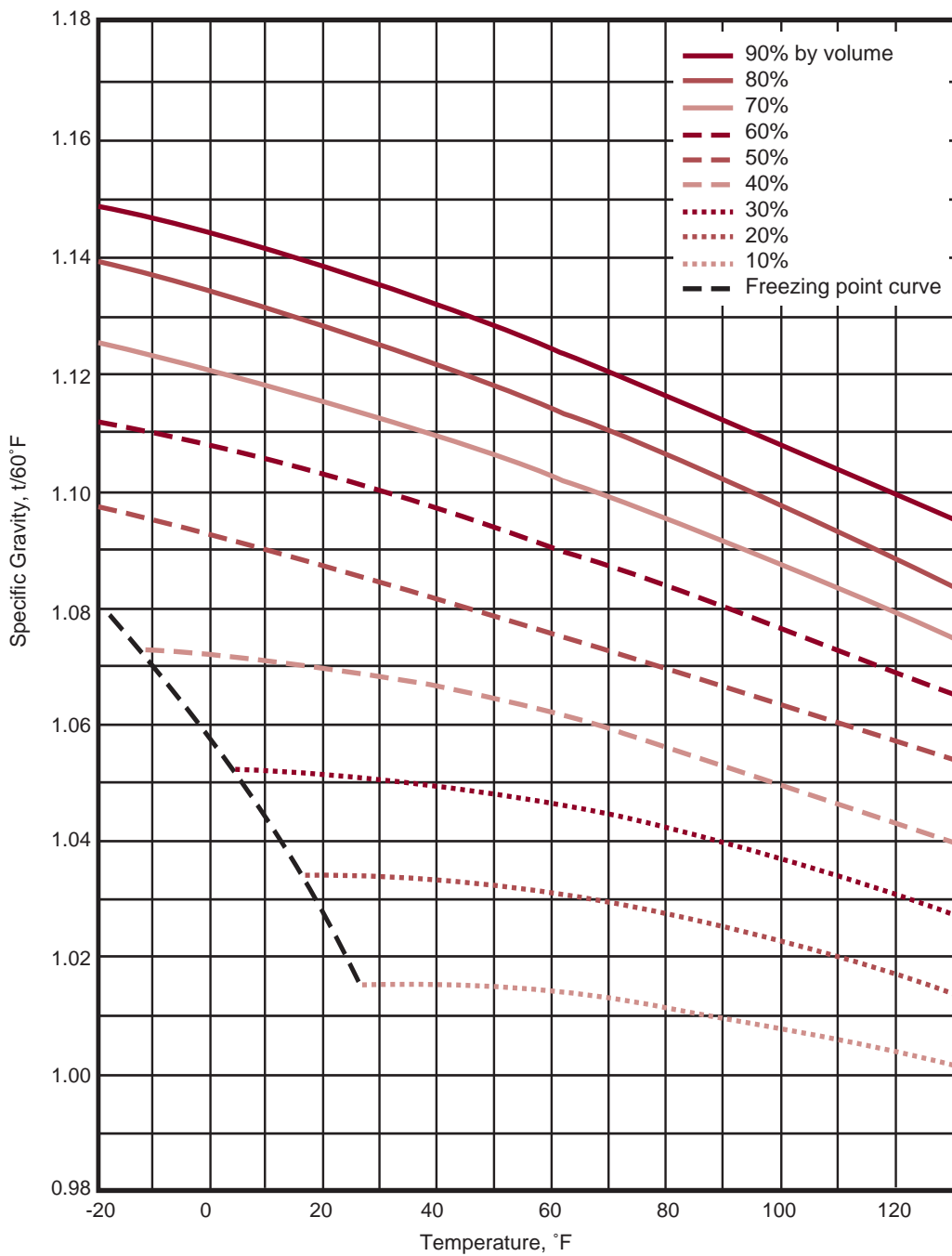
FIGURE 5 Specific Gravities of Aqueous Solutions of JEFFCOOL® E100 & E100N Coolants
